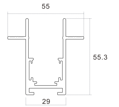
开槽宽: 30-32mm
